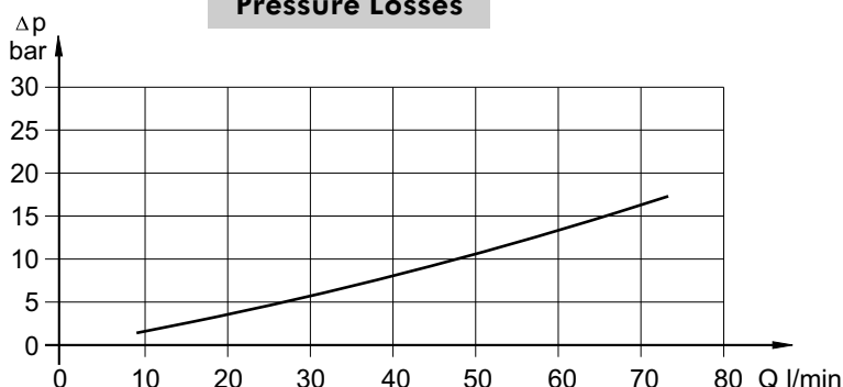
Pressure Losses
